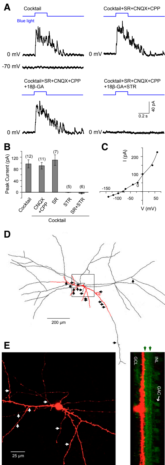
Fig. 1. Glycinergic synaptic input from GACs to PAS4/5 cells. (A) Responses of a voltage-clamped PAS4/5 cell to optogenetic (blue light) activation of GACs in physiological saline supplemented with a cocktail (20 \mu M L-AP4, 20 \mu M ACET, and 300 \mu M HEX), showing no response at -70 mV but outward currents at 0 mV (Upper Left) that were resistant to SR (50 \mu M), CNQX (40 \mu M), and CPP (20 \mu M) (Upper Right) and 18 \beta -GA (25 \mu M with 20 min perfusion; Lower Left) but were completely blocked by STR (1 \mu M; Lower Right). (B) Summary of peak response amplitudes at 0 mV in various receptor blockers shown in A. Numbers in parentheses, cells tested. (C) I-V curve of
