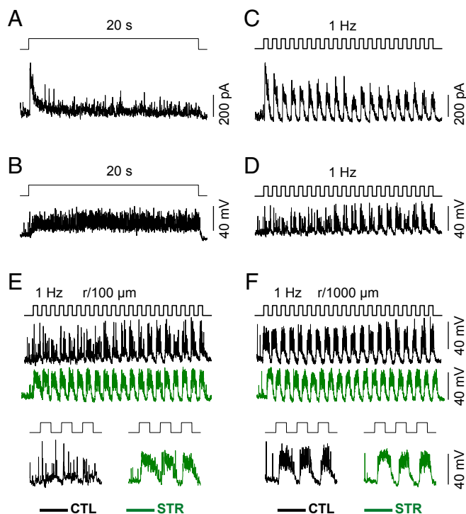
Fig. 4. Temporal dynamics of the glycinergic input to PAS4/5-1 cells. (A and B) Inhibitory current and voltage responses of a PAS4/5-1 to a prolonged (20-s) stimulation of a small (100- \mu\text{m} radius) center light spot, showing a transient inhibitory current input (A; voltage-clamped at 0 mV) and a transient suppression of spikes (B; current-clamped at the resting potential -74 mV) at the onset of the stimulation. (C and D) Responses to same duration of stimulation as in A and B but at a higher temporal frequency (1 Hz), showing repetitive bursts of inhibitory current inputs that persisted the entire stimulation duration (C) and repetitive bursts of spike responses that were suppressed at the onset of each burst (D). (E) The spike responses to the flickering small-spot stimulation in D (black trace) were greatly enhanced by STR (1 \mu\text{M} ; green trace), as shown more clearly in the expanded panels at the bottom, suggesting a significant suppression of spikes by a glycinergic drive in the control solution. (F) Responses to 1-Hz flickering of a large (1,000- \mu\text{m} radius) light spot, showing an increased spike rate in the control solution (black trace) compared to the response to the small flickering spot (D) and a lack of significant effect of STR on the spike rate (green trace), as seen more clearly in the expanded panels at the bottom.
