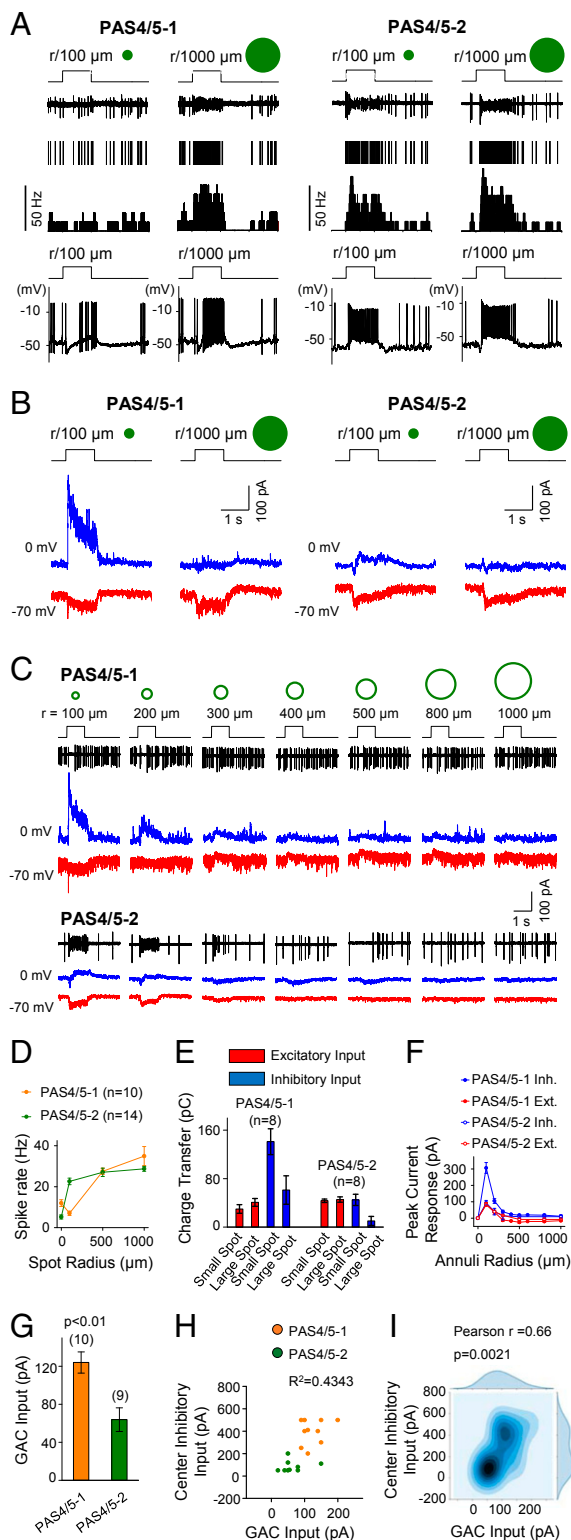
Fig. 2. Receptive field properties and synaptic connectivity of two subtypes of PAS4/5 cells. (A) (Top) Visual responses of a PAS4/5-1 and a PAS4/5-2 to small (100- \mu\text{m} radius) and large (1,000- \mu\text{m} radius) light spot illumination under on-cell loose-patch recording (first three rows show spike trains, raster plots, and spike rates, respectively) and whole-cell current-clamp recording (fourth row), showing transient sbc receptive field properties in the PAS4/5-1 but not the PAS4/5-2 cell. (B) Responses of a PAS4/5-1 and a PAS4/5-2 to small and large light spot illumination under whole-cell voltage clamp at 0 mV (blue) and -70 mV (red). (C) Responses of a PAS4/5-1 and a PAS4/5-2 to light annuli of various radii under on-cell loose-patch (Top) and whole-cell
